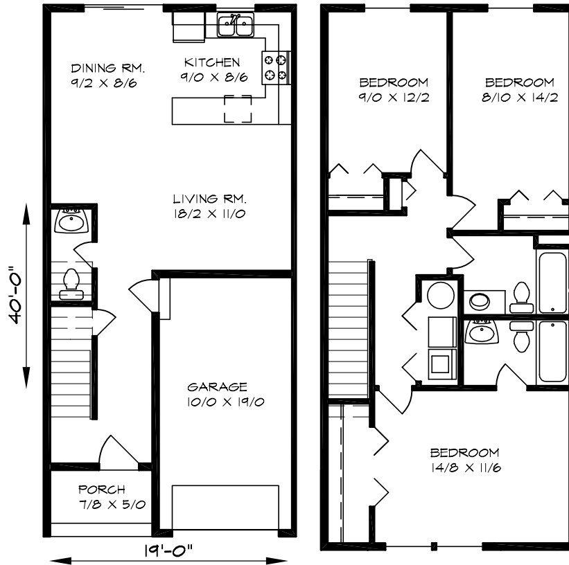
MAIN FLOOR
