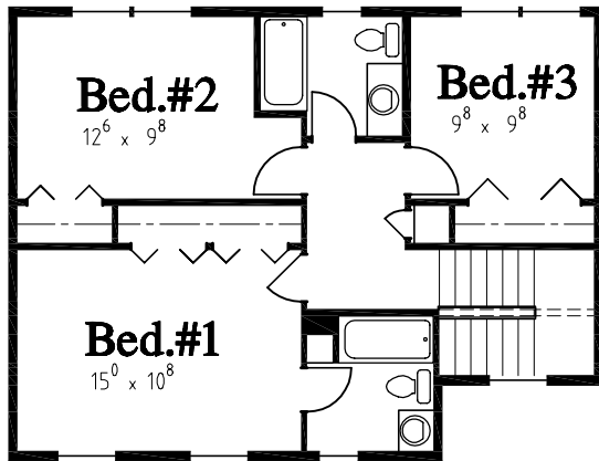
UPPER FLOOR
