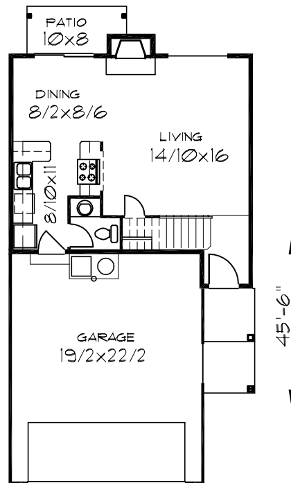
25'-0" EACH UNIT MAIN FLOOR PLAN
