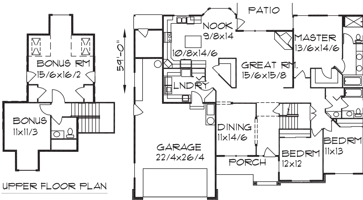
65'-0" MAIN FLOOR PLAN
