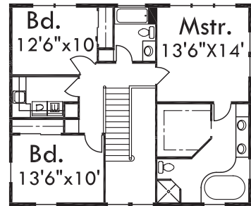
UPPER FLOOR
