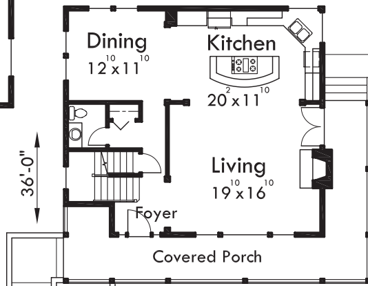
MAIN FLOOR
