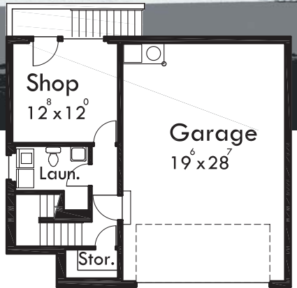
LOWER FLOOR
