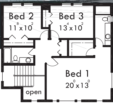
UPPER FLOOR
