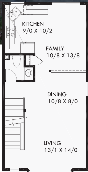
2nd Floor
