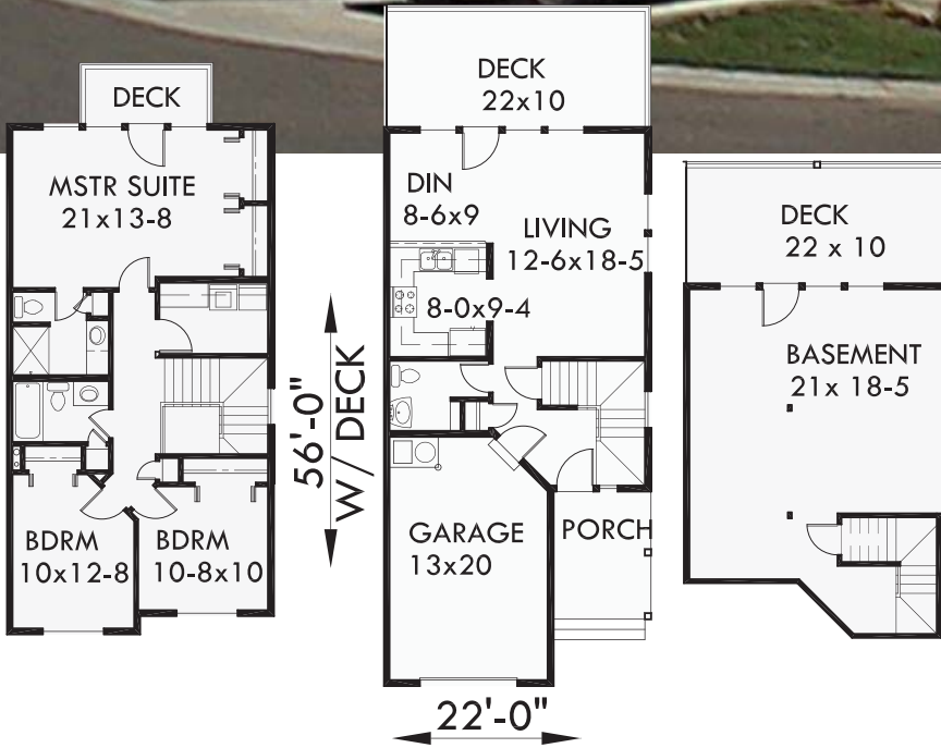
UPPER FLOOR
