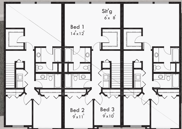
UPPER FLOOR
