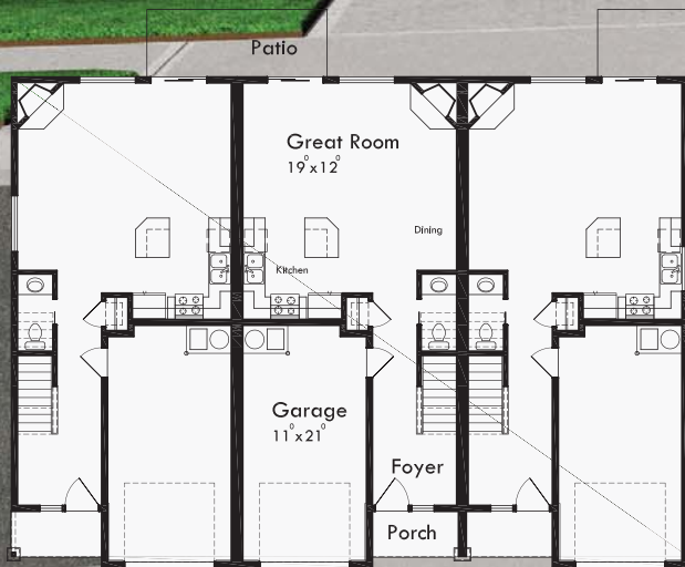
← 20'-0" per unit → MAIN FLOOR
