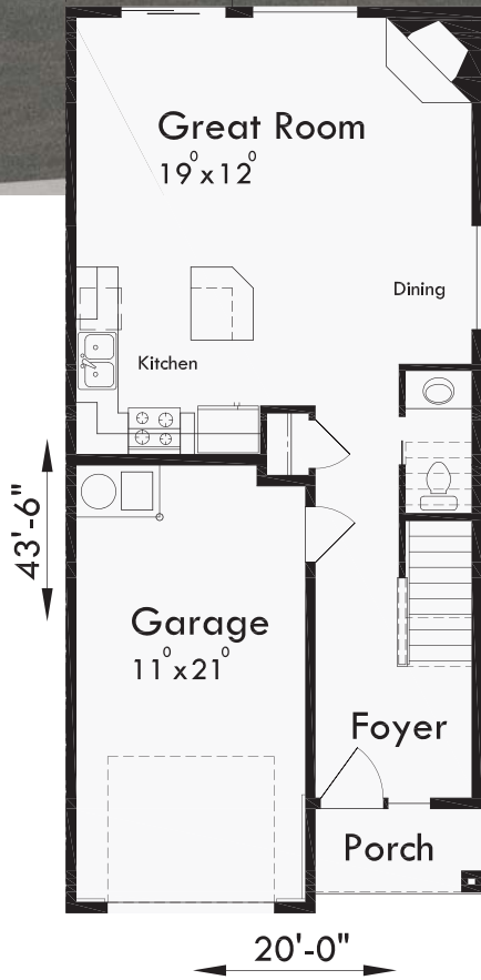
MAIN FLOOR
