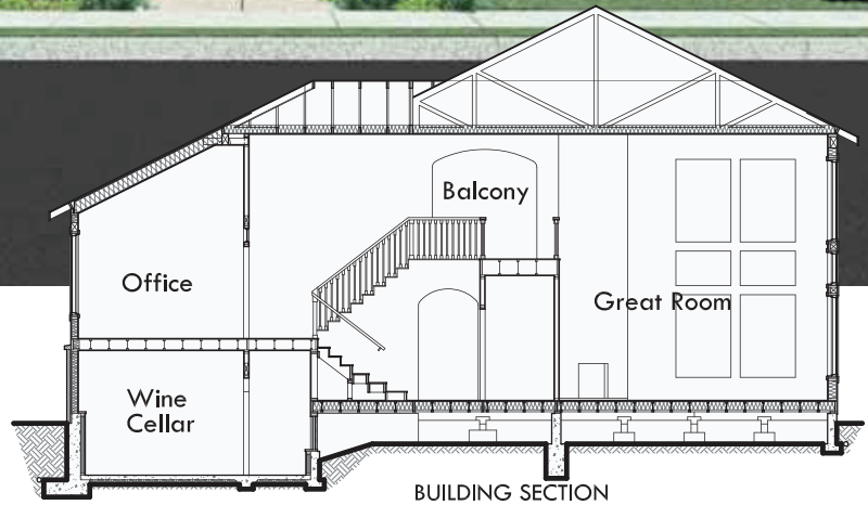
BUILDING SECTION
