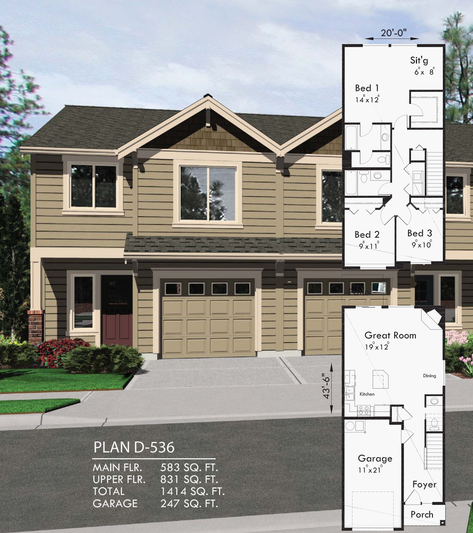
MAIN FLOOR
