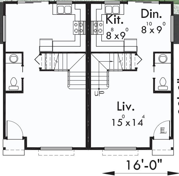
MAIN FLOOR
