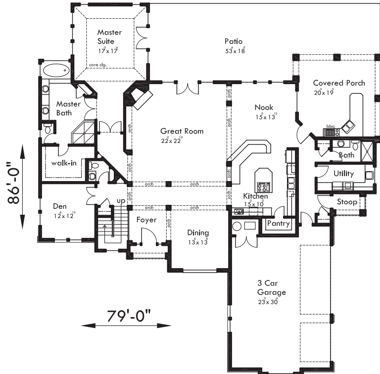
MAIN FLOOR
